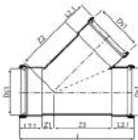
45° Y (Tee) Branch (3 Socket)
