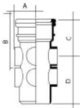
Unequal Branch (6 way bossed pipe. All bosses molded solid)
