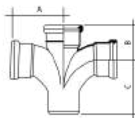
Cross Tee 87.5°
