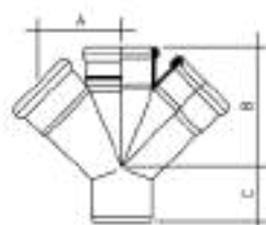
Double Branch 45°
