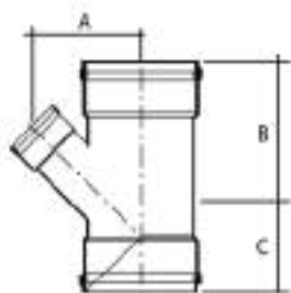
Y Branch 45° (Reducing)
