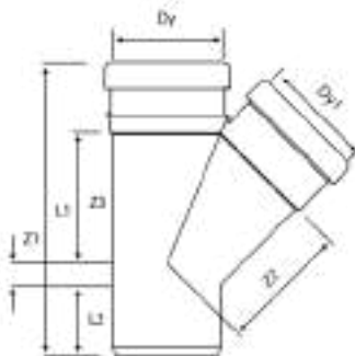
45° Y (Tee) Branch (2 Socket / Spigot )
