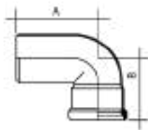
Horizontal Outlet W.C. Pan Connector 90° (One plain end)
